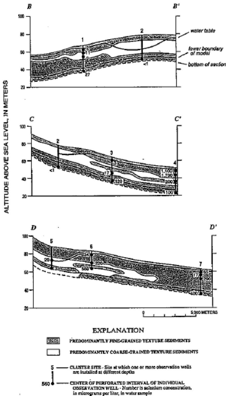
Figure 222 Cross-sectional diagram showing selenium concentrations in observation well samples and texture of deposits (Deverel et al., 1994, p. 177).
