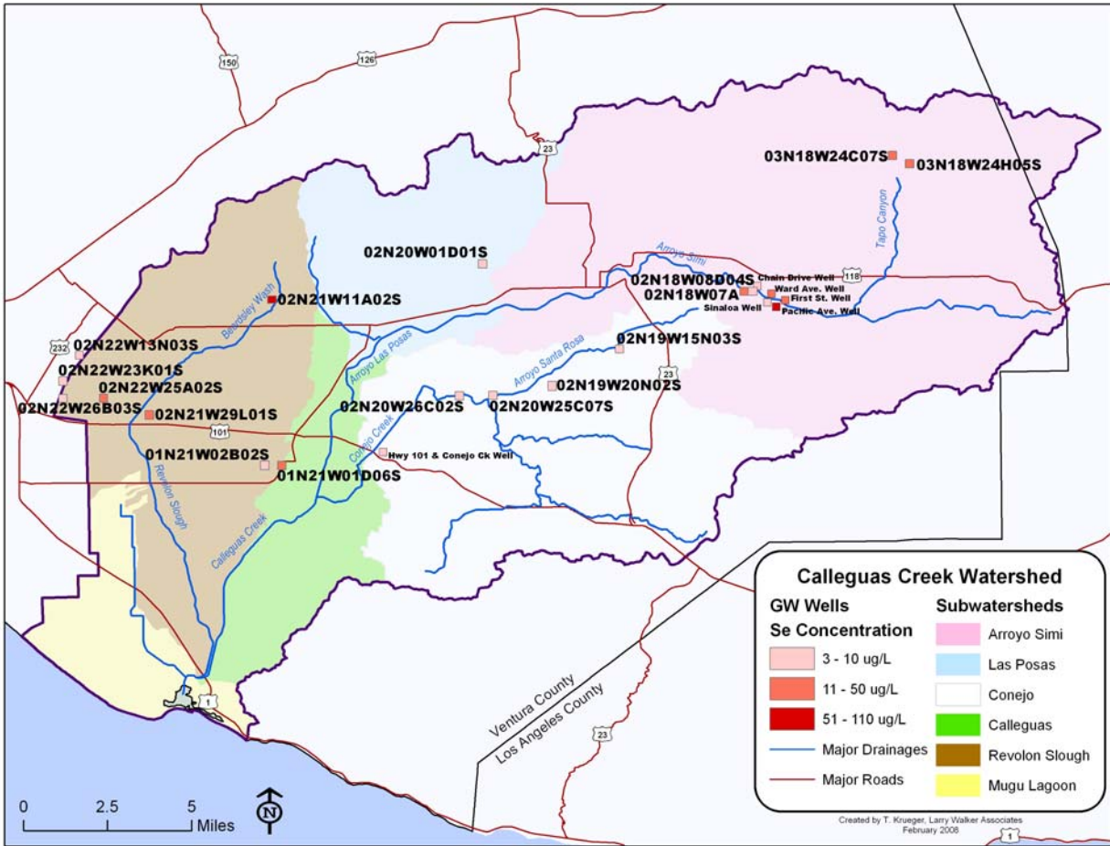
Figure 333 Map of the available selenium data in the Calleguas watershed. The wells located in the Simi Valley area are dewatering wells and they were presented in the Metals TMDL report (LWA, 2006, p. 79).
